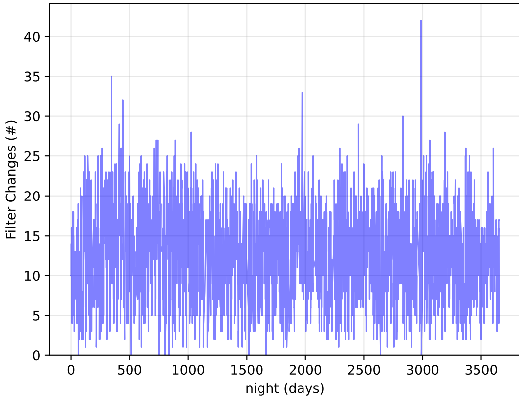
too_elab_heavy_r64_d2_griz_v3.4_10yrs Per Night: Filter Changes
