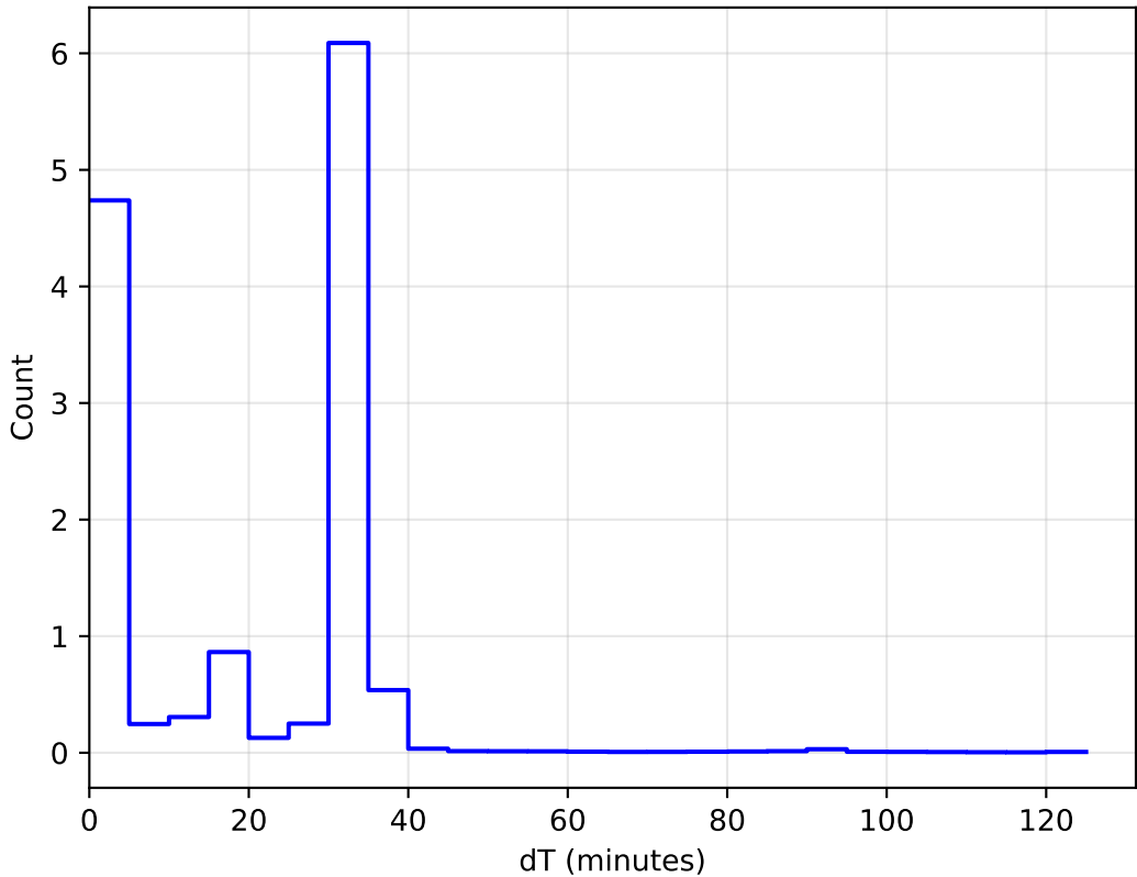
too_elab_heavy_r64_d2_griz_v3.4_10yrs All sky: DeltaT Histogram 1e6
