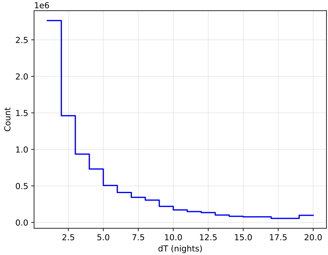
too_elab_heavy_r64_d2_griz_v3.4_10yrs All sky all bands: DeltaNight Histogram
