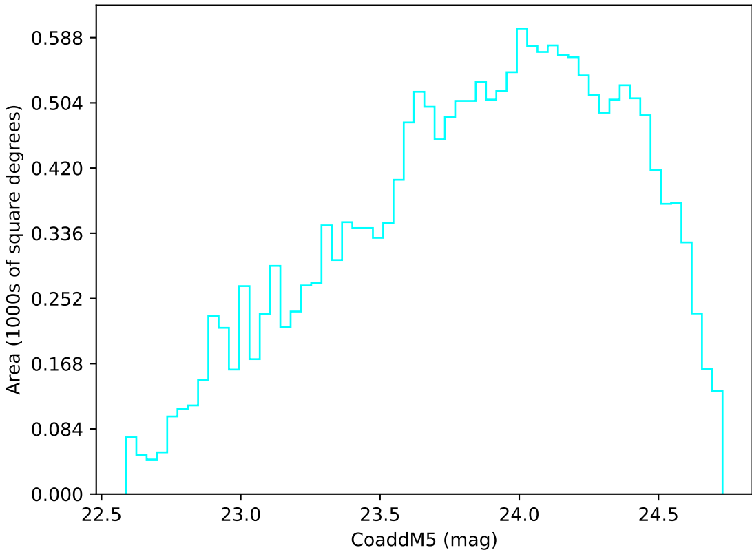
too_elab_heavy_r64_d2_griz_v3.4_10yrs Yr 3-4 u band: CoaddM5
