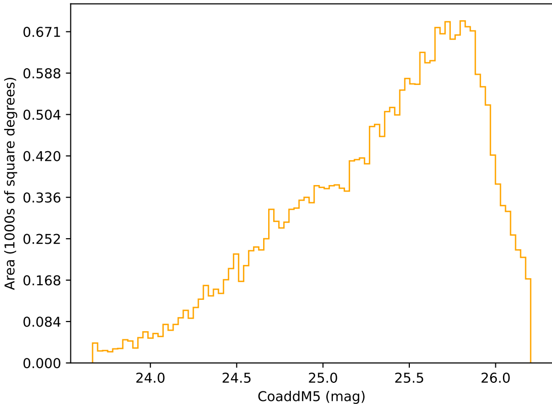
too_elab_heavy_r64_d2_griz_v3.4_10yrs Yr 3-4 r band: CoaddM5
