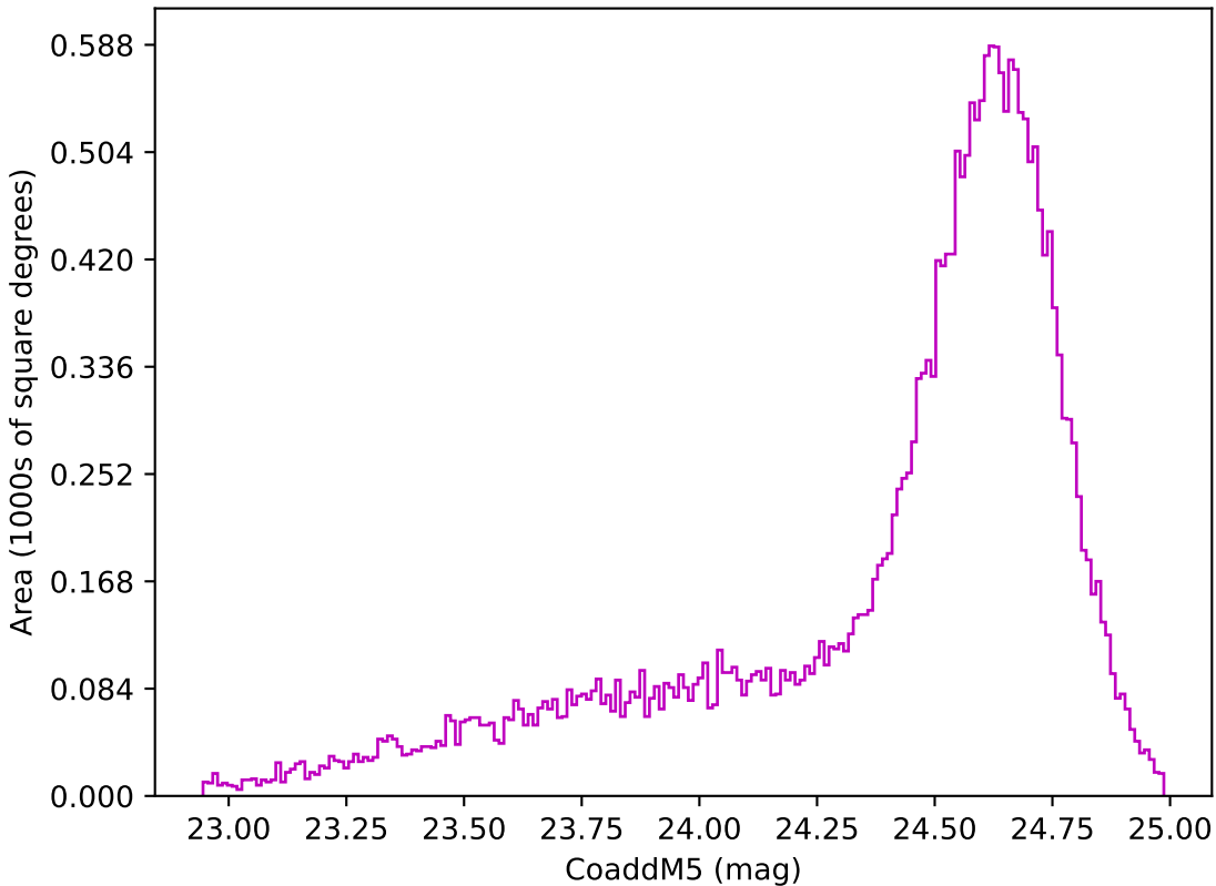
too_elab_heavy_r64_d2_griz_v3.4_10yrs Yr 1 z band: CoaddM5
