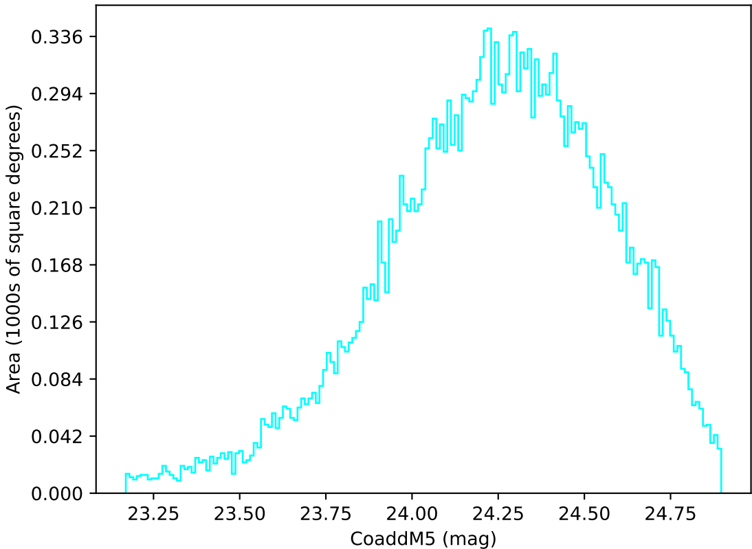
too_elab_heavy_r64_d2_griz_v3.4_10yrs Yr 1 u band: CoaddM5
