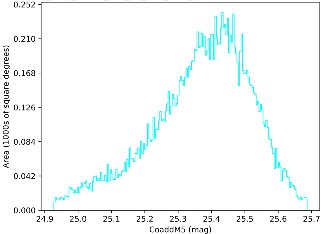
too_elab_heavy_r64_d2_griz_v3.4_10yrs WFD u band: CoaddM5
