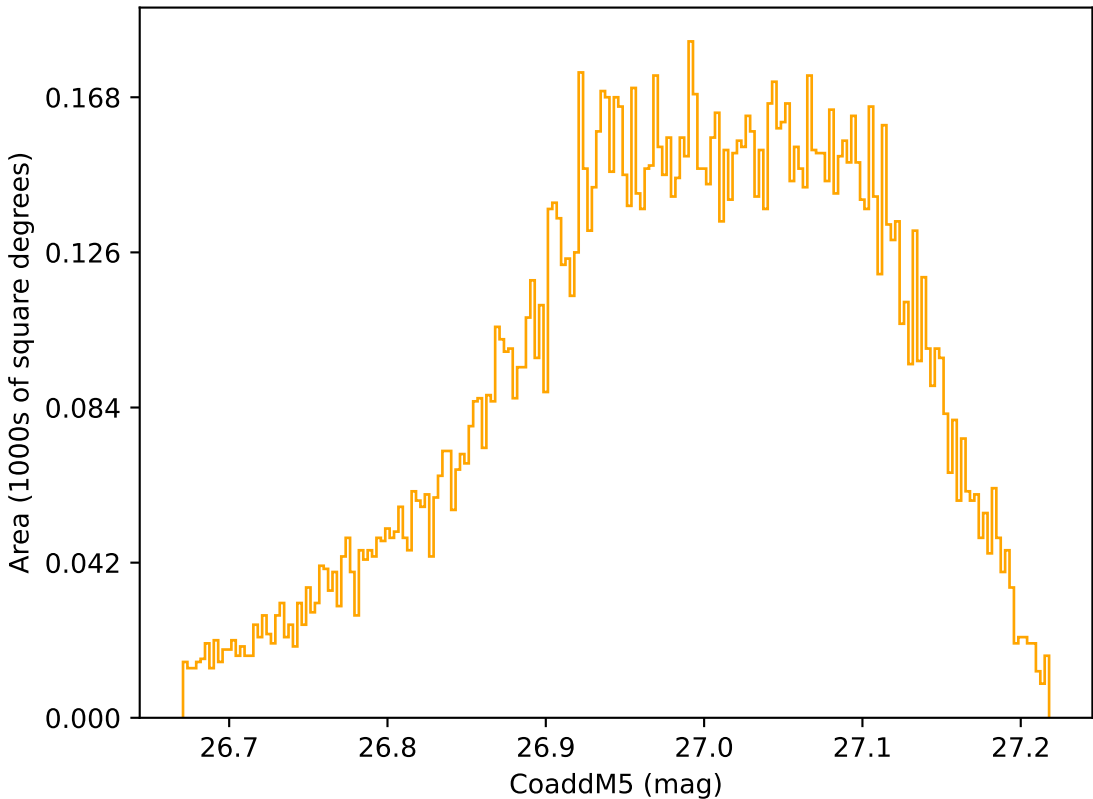
too_elab_heavy_r64_d2_griz_v3.4_10yrs WFD r band: CoaddM5
