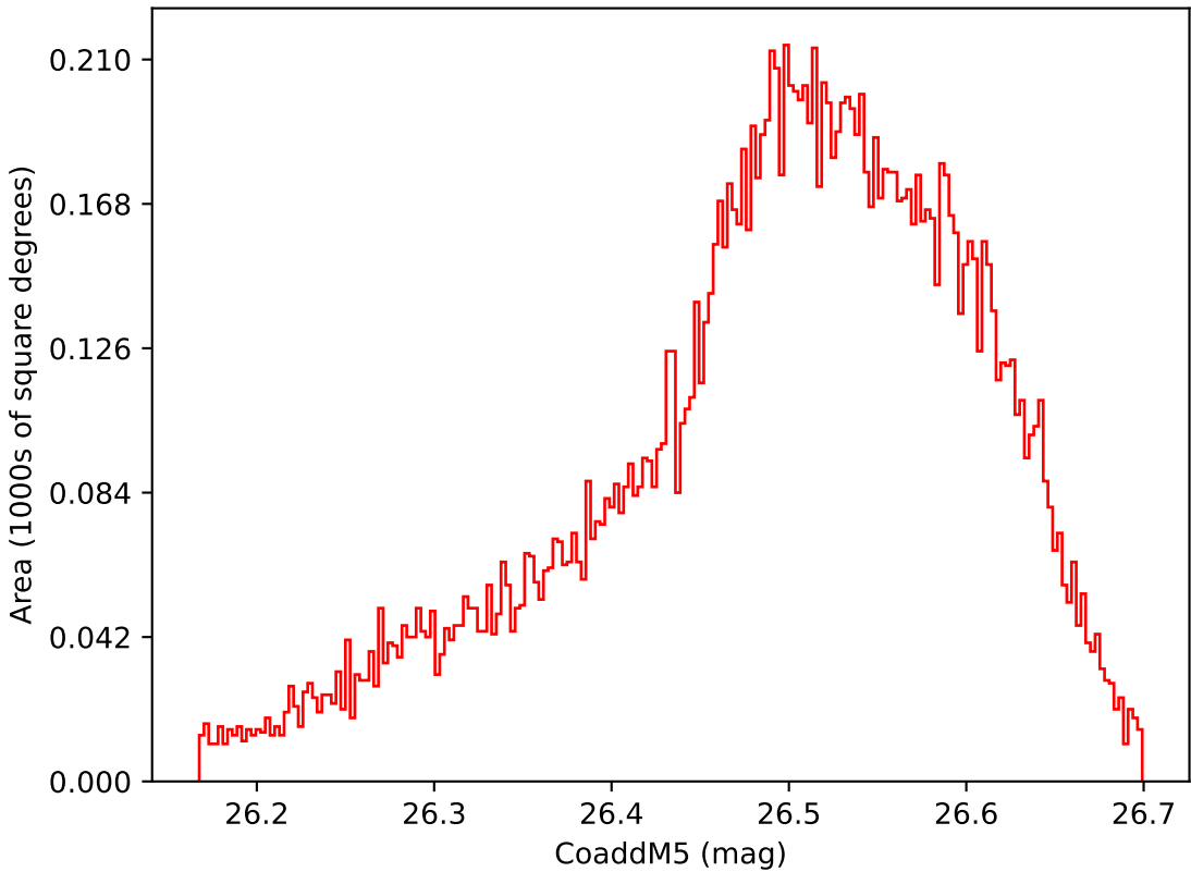
too_elab_heavy_r64_d2_griz_v3.4_10yrs WFD i band: CoaddM5
