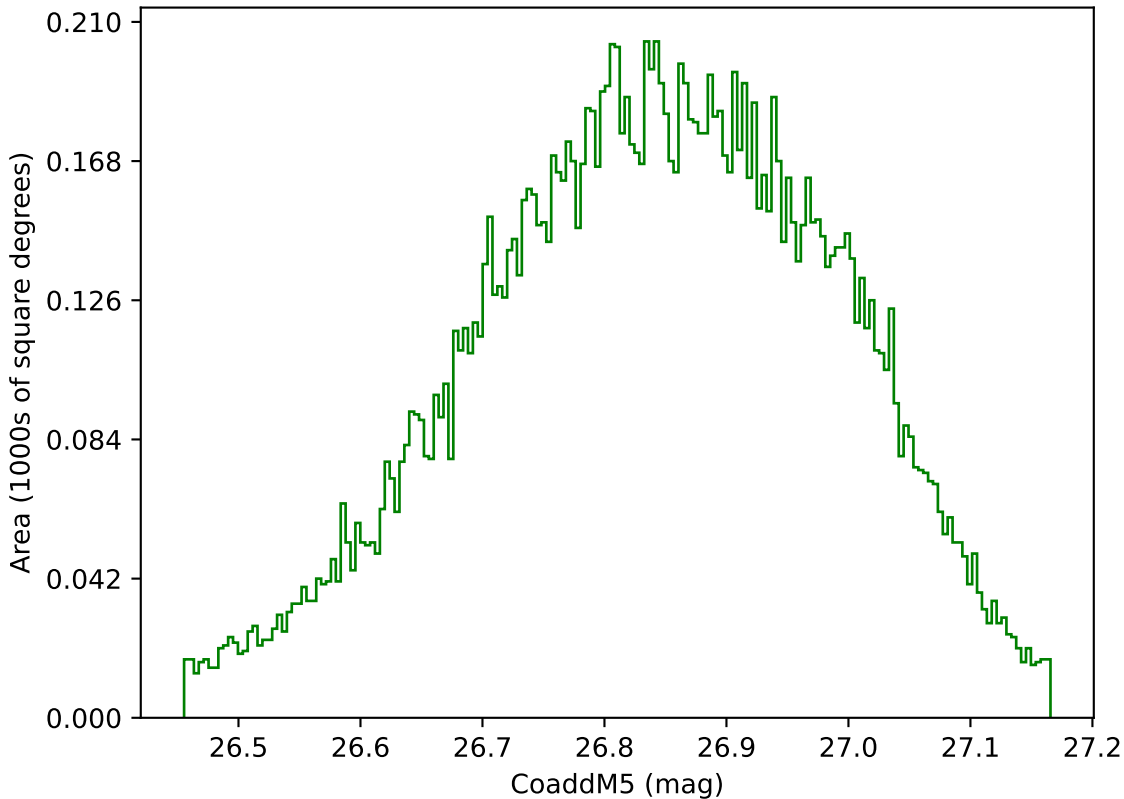
too_elab_heavy_r64_d2_griz_v3.4_10yrs WFD g band: CoaddM5
