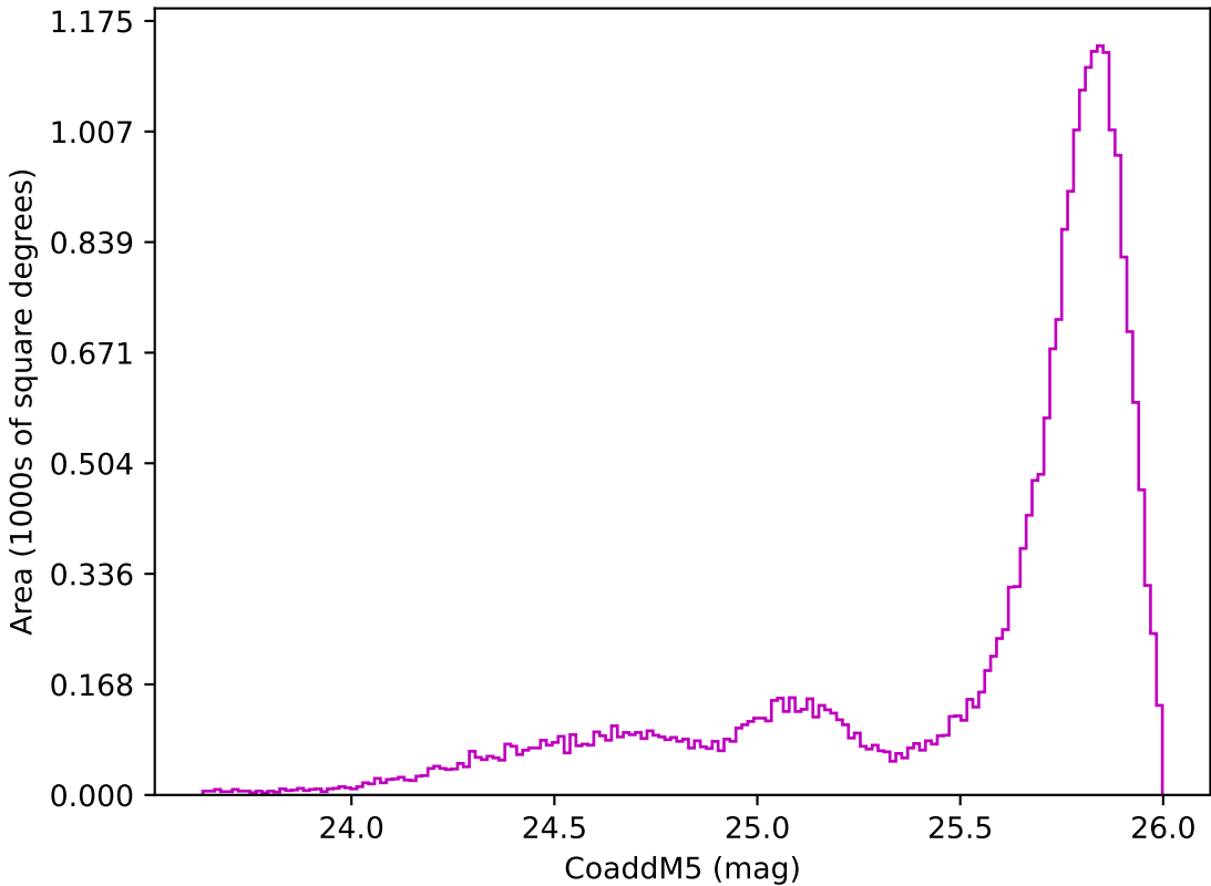
too_elab_heavy_r64_d2_griz_v3.4_10yrs All sky z band: CoaddM5
