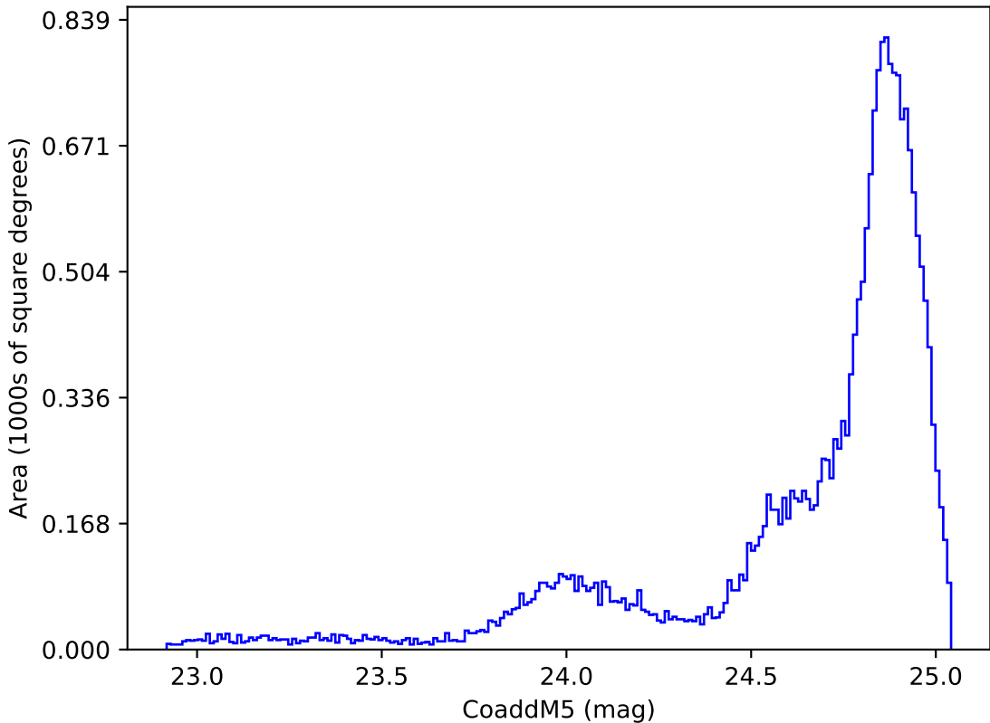
too_elab_heavy_r64_d2_griz_v3.4_10yrs All sky y band: CoaddM5
