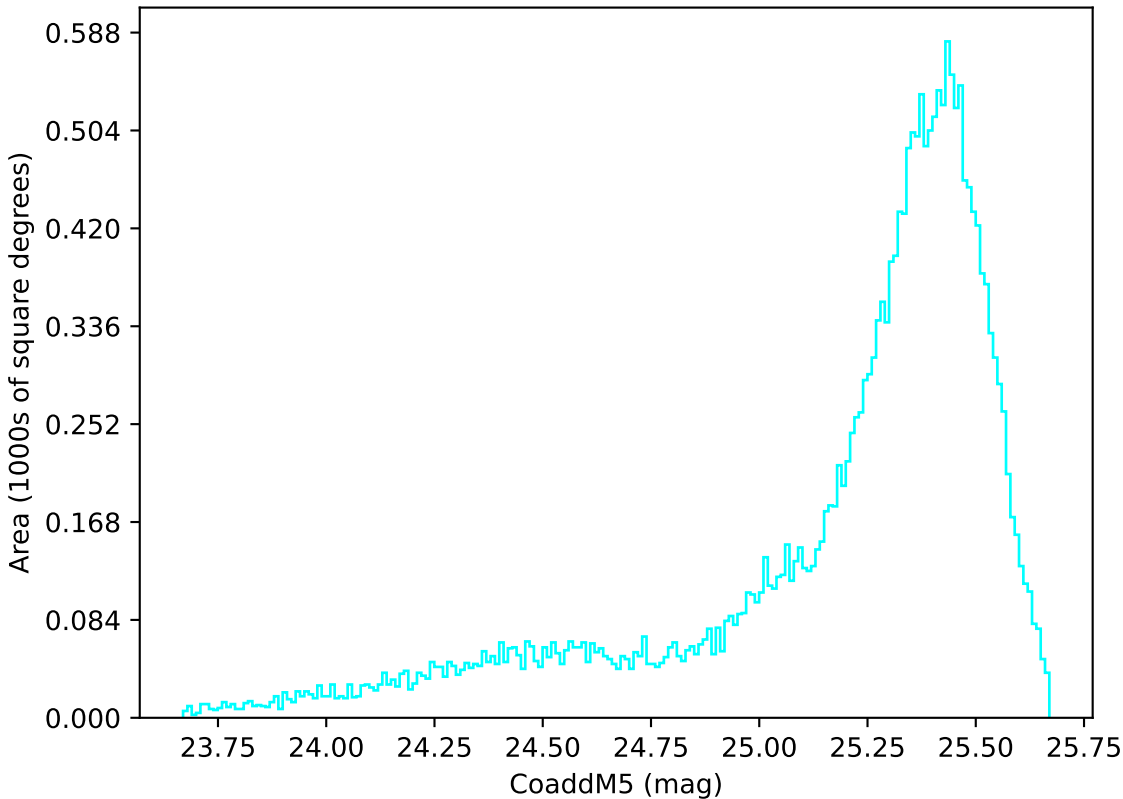
too_elab_heavy_r64_d2_griz_v3.4_10yrs All sky u band: CoaddM5
