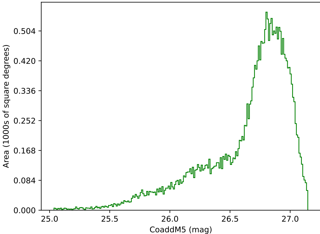
too_elab_heavy_r64_d2_griz_v3.4_10yrs All sky g band: CoaddM5
