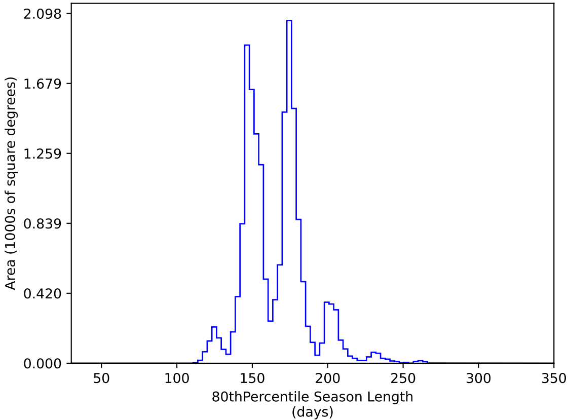
too_elab_heavy_r64_d2_griz_v3.4_10yrs WFD y band: 80thPercentile Season Length
