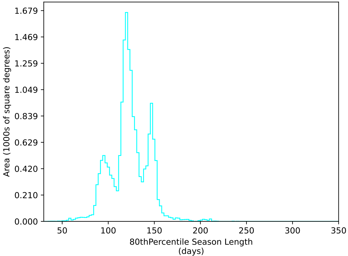
too_elab_heavy_r64_d2_griz_v3.4_10yrs WFD u band: 80thPercentile Season Length
