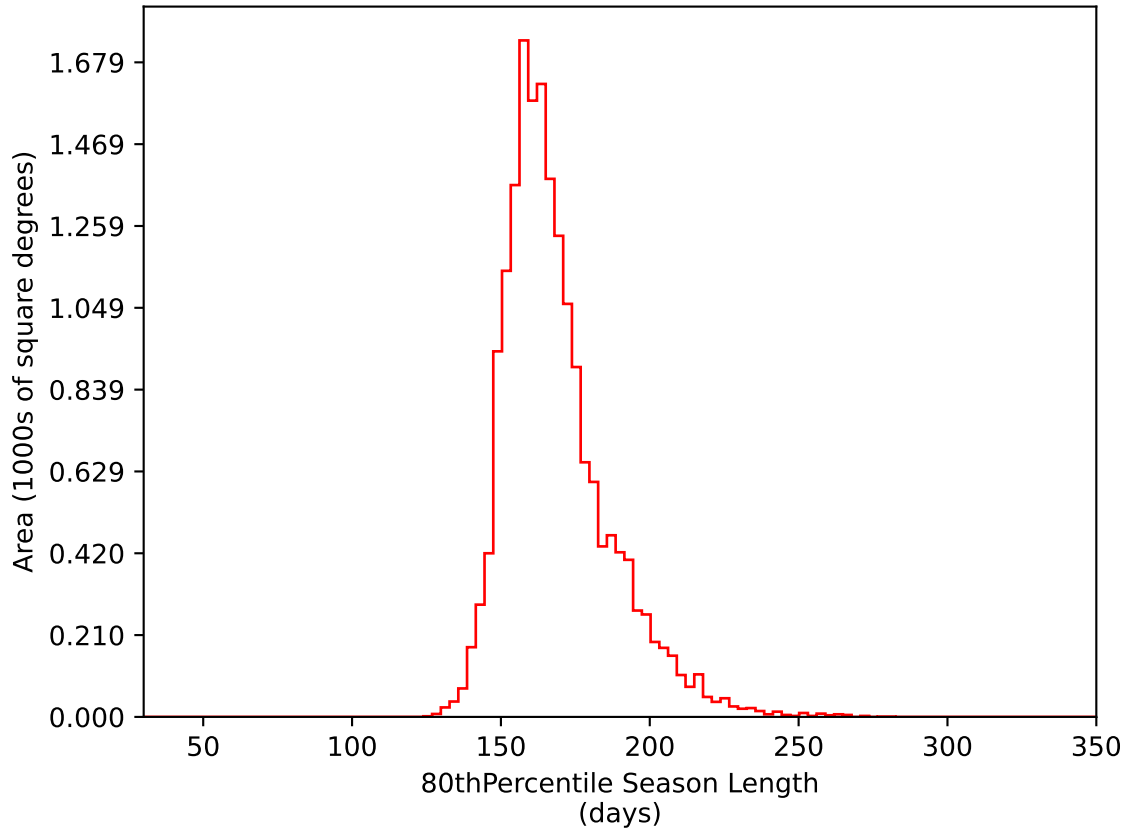
too_elab_heavy_r64_d2_griz_v3.4_10yrs WFD i band: 80thPercentile Season Length
