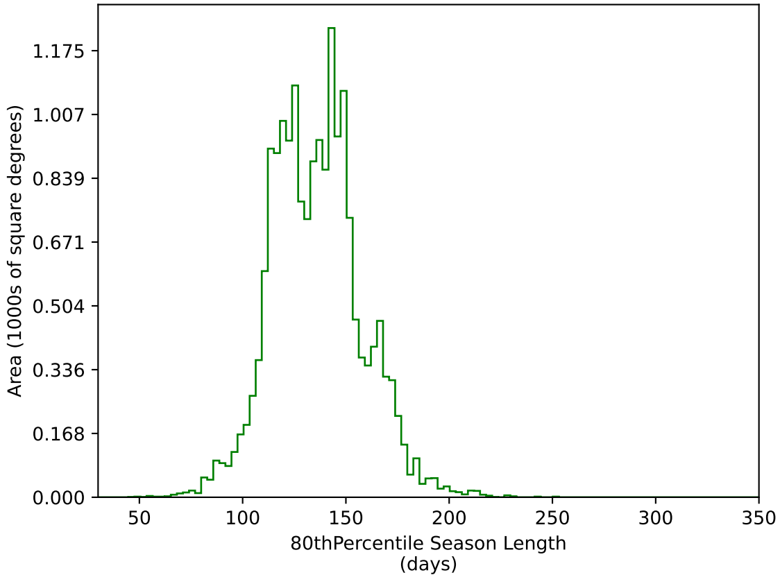
too_elab_heavy_r64_d2_griz_v3.4_10yrs WFD g band: 80thPercentile Season Length
