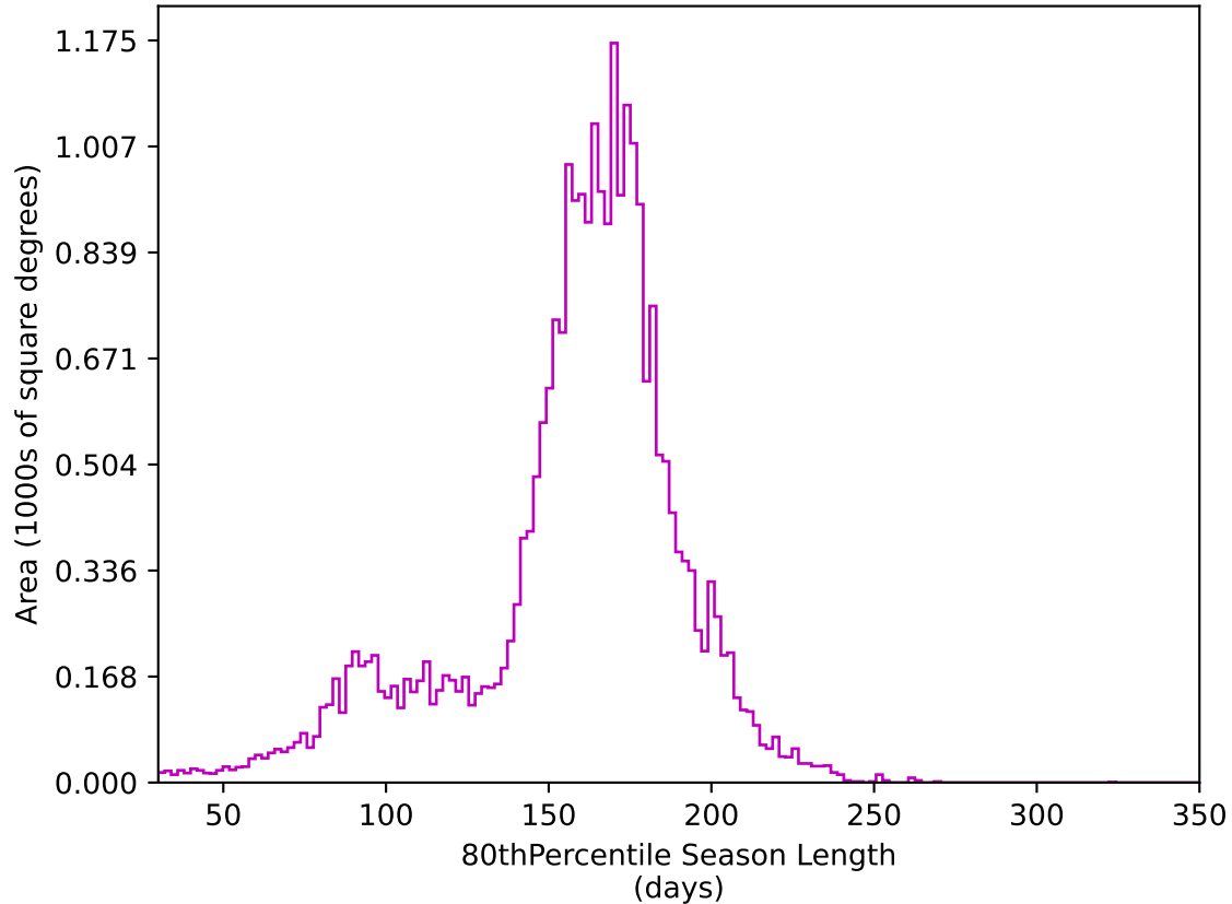
too_elab_heavy_r64_d2_griz_v3.4_10yrs All sky z band: 80thPercentile Season Length
