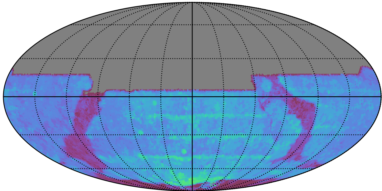
too_elab_heavy_r64_d2_griz_v3.4_10yrs All sky y band: 80thPercentile Season Length
