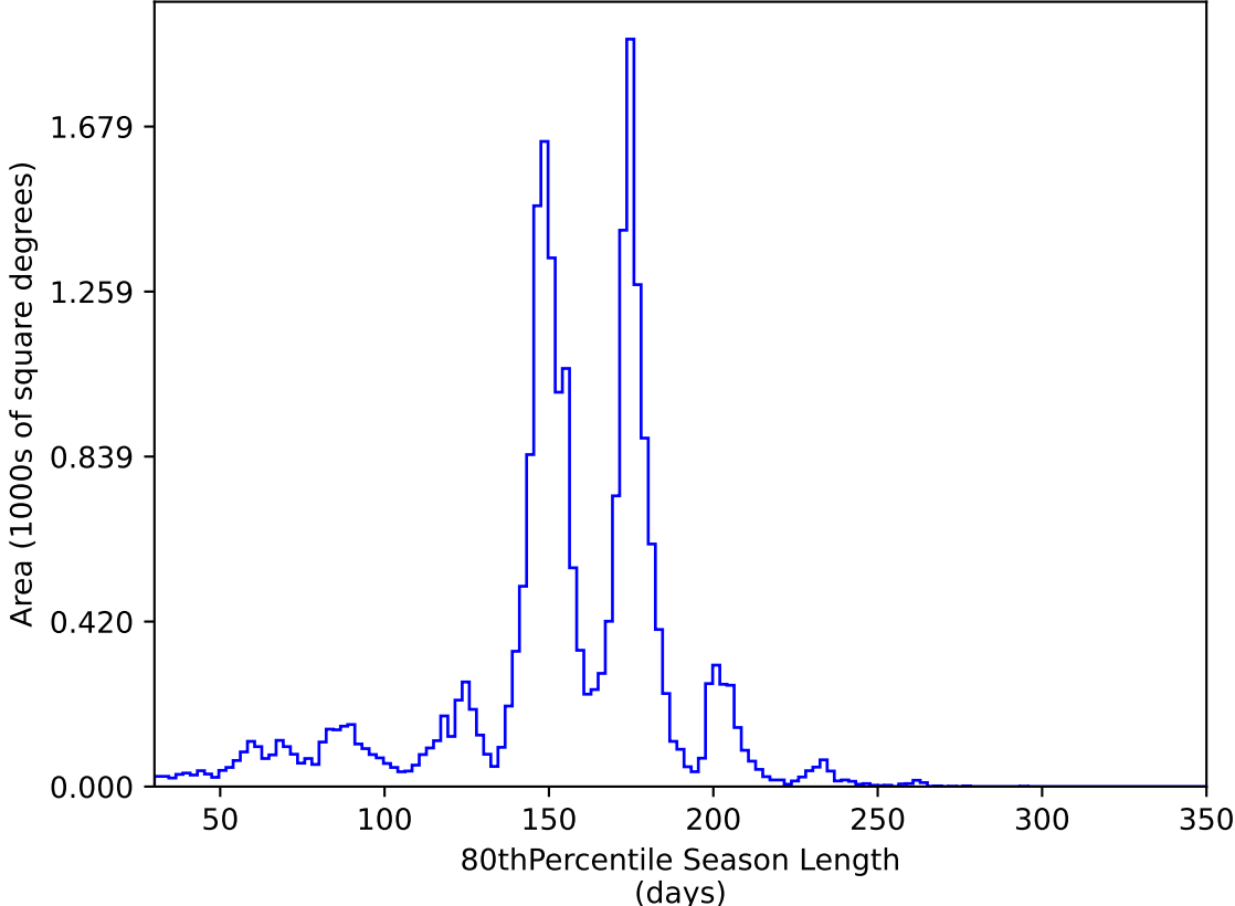
too_elab_heavy_r64_d2_griz_v3.4_10yrs All sky y band: 80thPercentile Season Length
