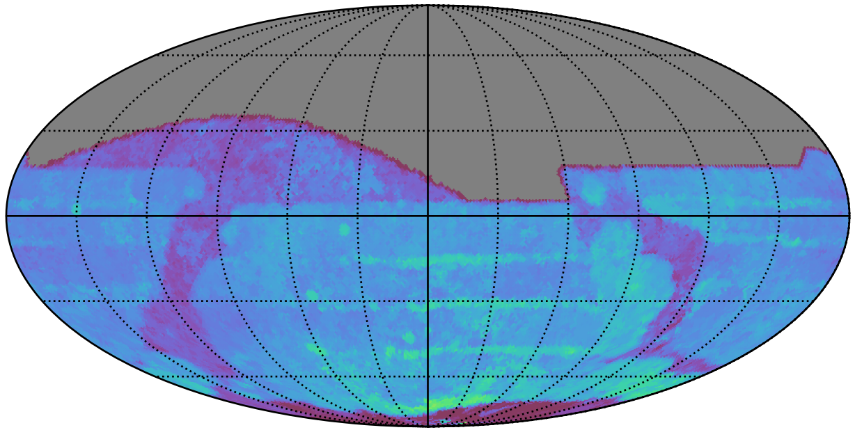
too_elab_heavy_r64_d2_griz_v3.4_10yrs All sky r band: 80thPercentile Season Length
