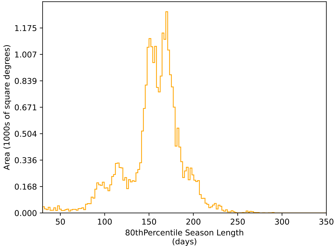
too_elab_heavy_r64_d2_griz_v3.4_10yrs All sky r band: 80thPercentile Season Length
