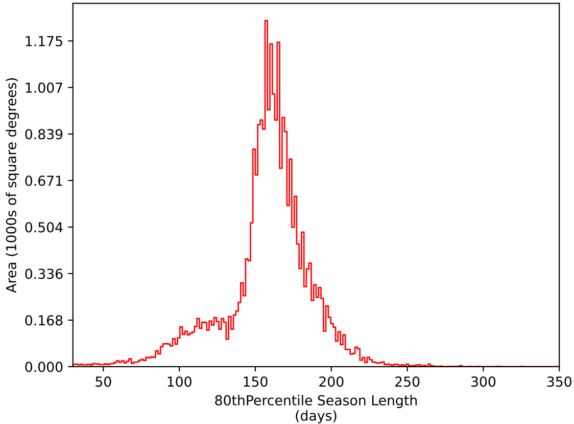
too_elab_heavy_r64_d2_griz_v3.4_10yrs All sky i band: 80thPercentile Season Length
