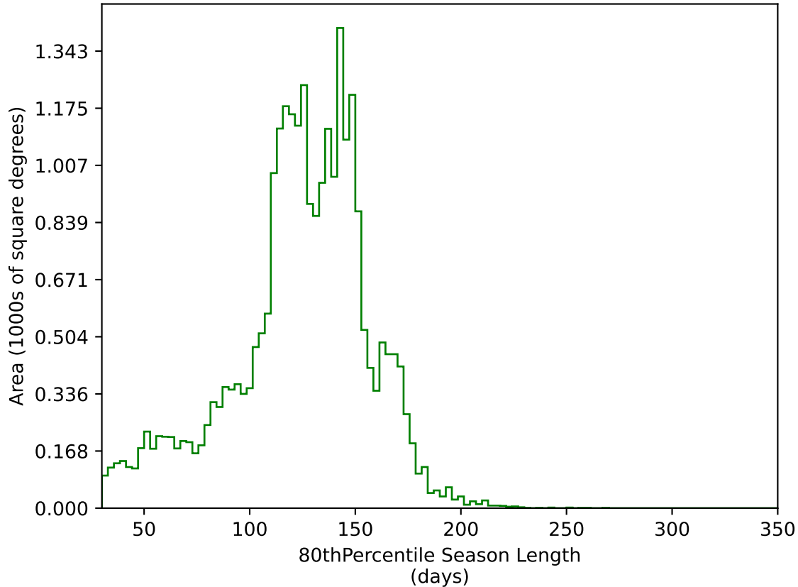
too_elab_heavy_r64_d2_griz_v3.4_10yrs All sky g band: 80thPercentile Season Length
