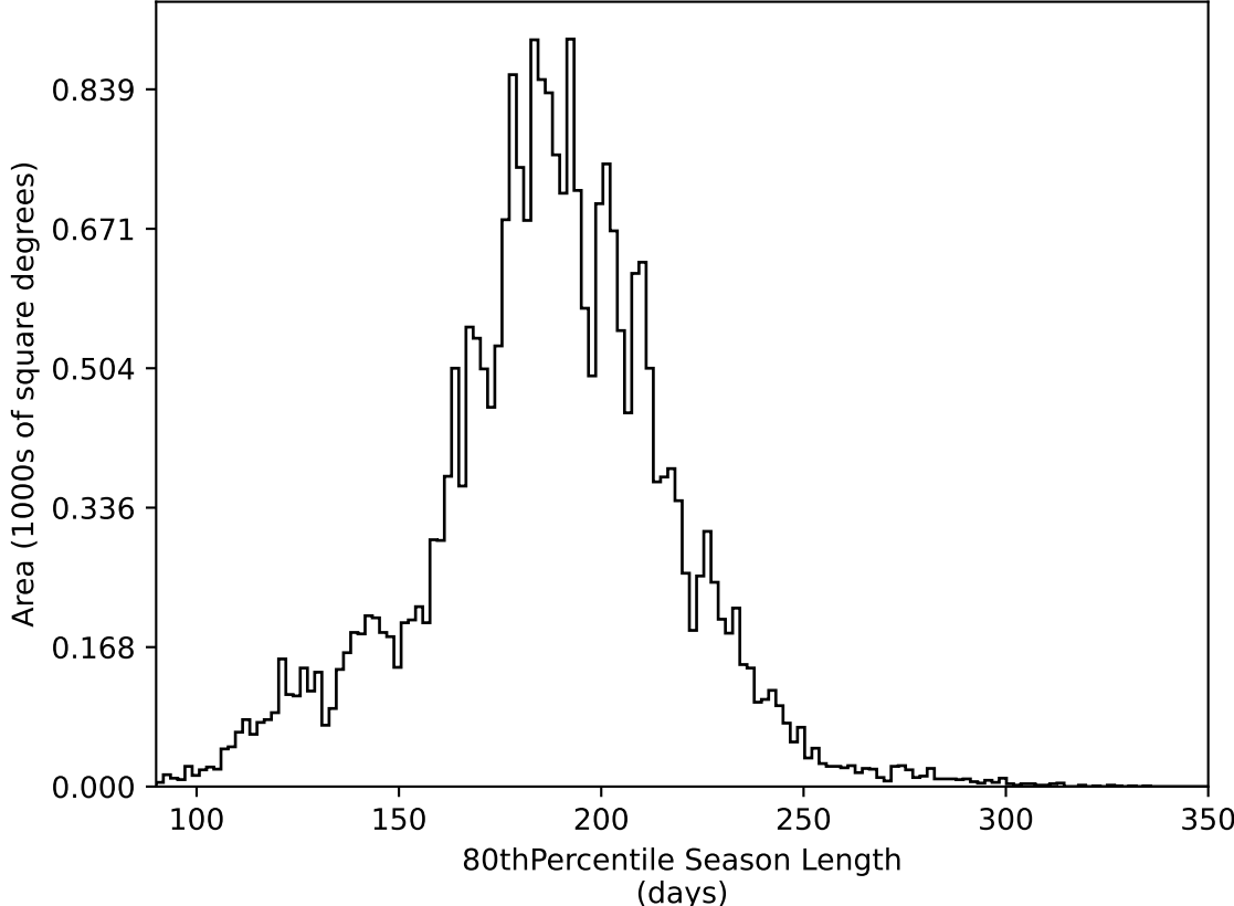
too_elab_heavy_r64_d2_griz_v3.4_10yrs All sky all bands: 80thPercentile Season Length
