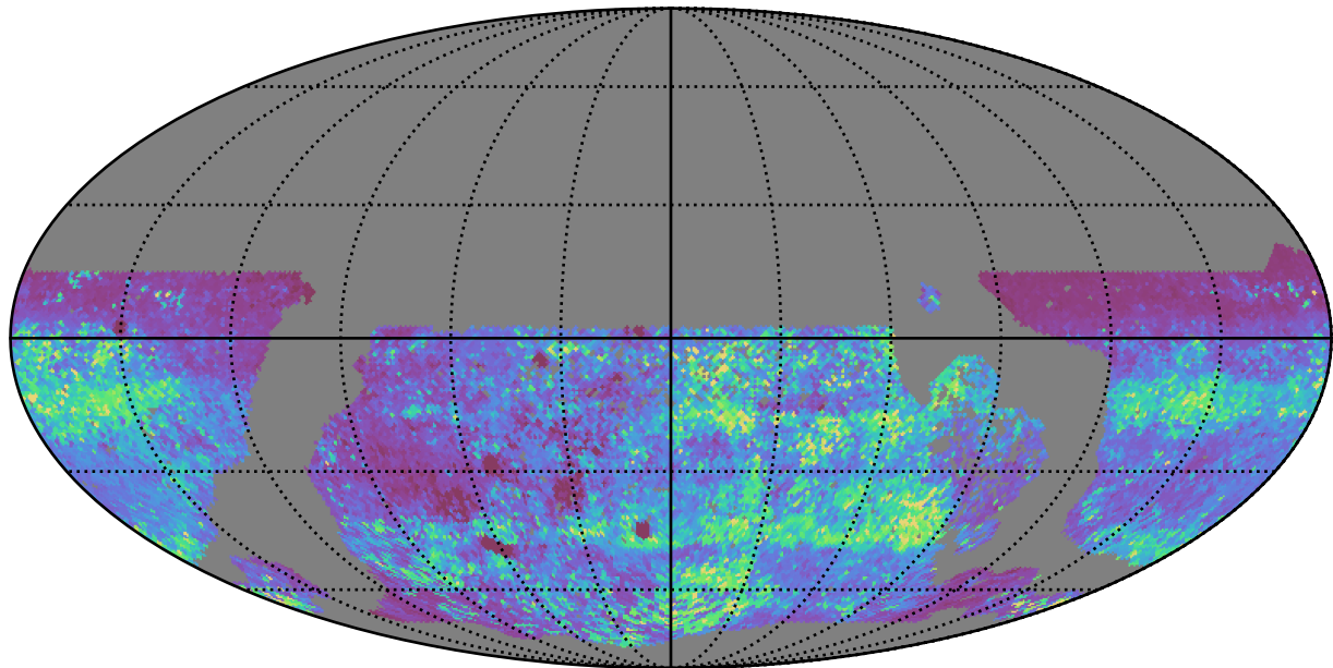
too_elab_heavy_r64_d2_griz_v3.4_10yrs WFD zy bands: 75th Percentile Intranight Timespan
