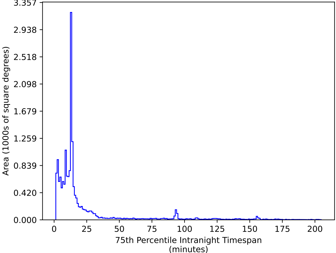
too_elab_heavy_r64_d2_griz_v3.4_10yrs WFD z band: 75th Percentile Intranight Timespan
