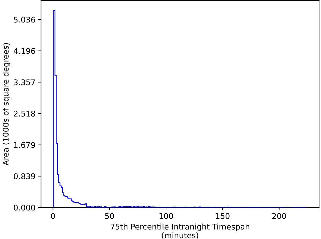
too_elab_heavy_r64_d2_griz_v3.4_10yrs WFD u band: 75th Percentile Intranight Timespan
