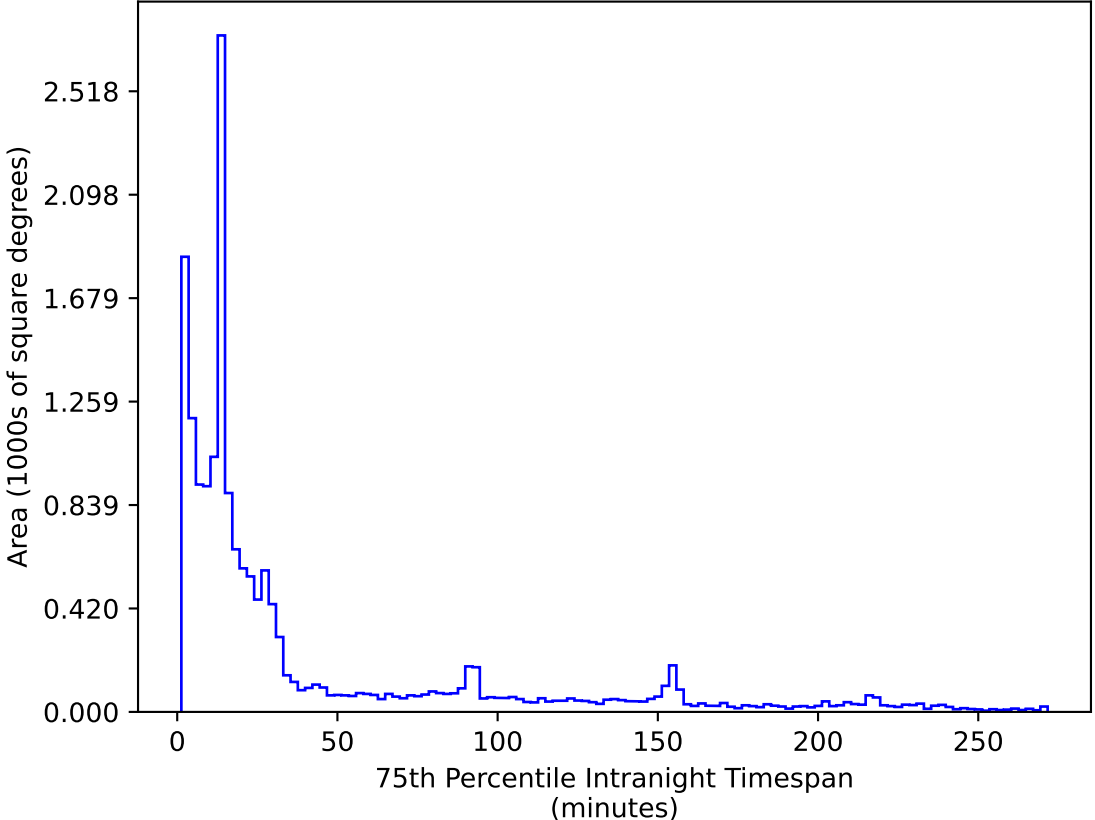
too_elab_heavy_r64_d2_griz_v3.4_10yrs WFD r band: 75th Percentile Intranight Timespan
