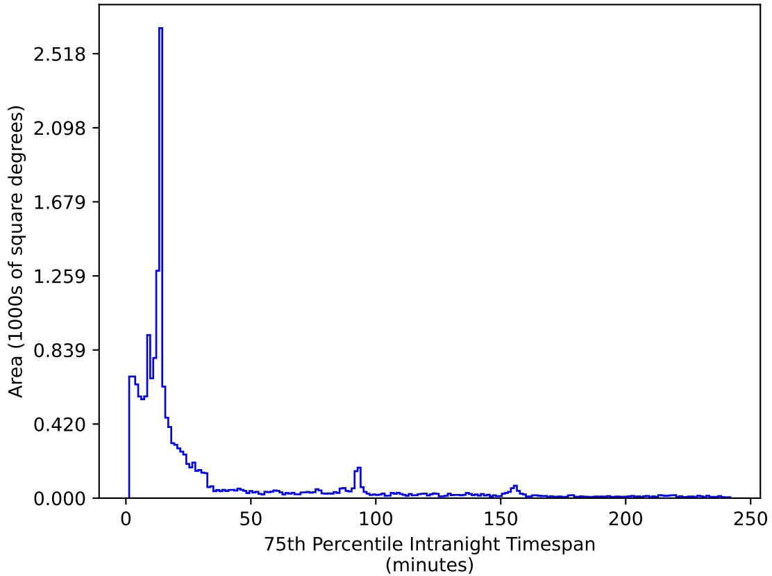
too_elab_heavy_r64_d2_griz_v3.4_10yrs WFD i band: 75th Percentile Intranight Timespan
