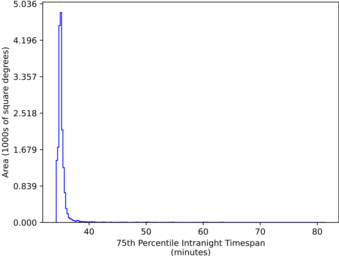
too_elab_heavy_r64_d2_griz_v3.4_10yrs WFD gr bands: 75th Percentile Intranight Timespan
