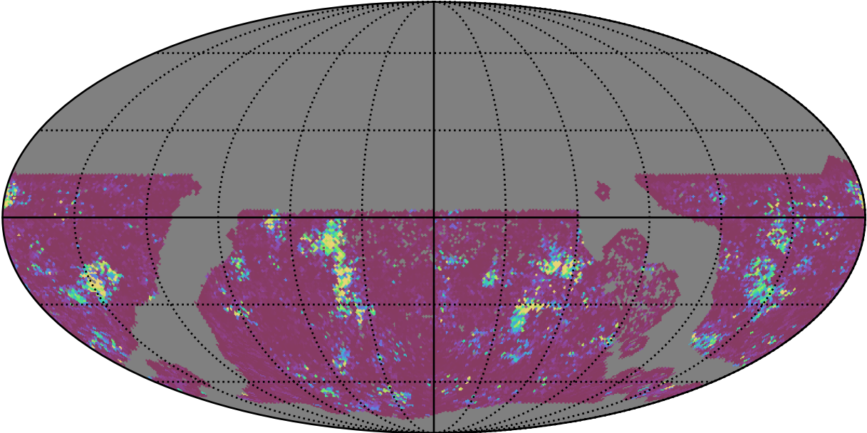
too_elab_heavy_r64_d2_griz_v3.4_10yrs WFD g band: 75th Percentile Intranight Timespan
