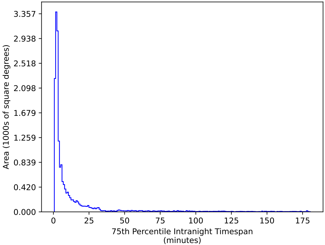
too_elab_heavy_r64_d2_griz_v3.4_10yrs WFD g band: 75th Percentile Intranight Timespan
