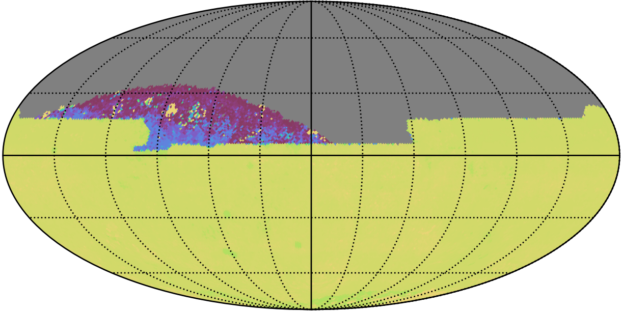
too_elab_heavy_r64_d2_griz_v3.4_10yrs All sky zy bands: 75th Percentile Intranight Timespan
