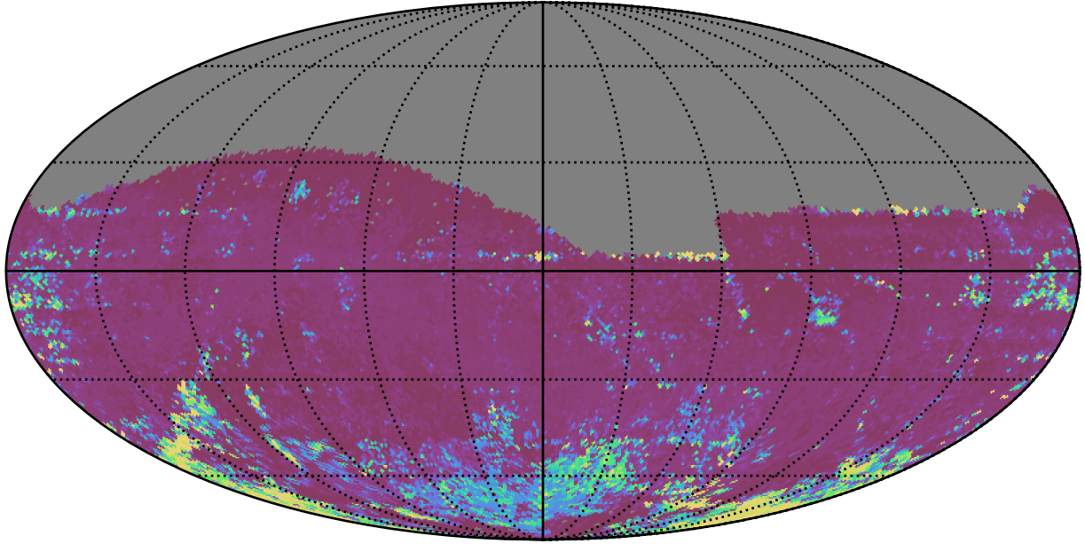
too_elab_heavy_r64_d2_griz_v3.4_10yrs All sky z band: 75th Percentile Intranight Timespan
