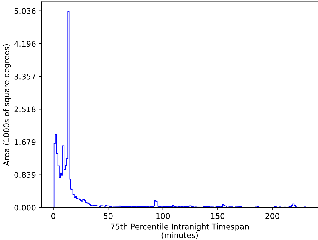
too_elab_heavy_r64_d2_griz_v3.4_10yrs All sky z band: 75th Percentile Intranight Timespan
