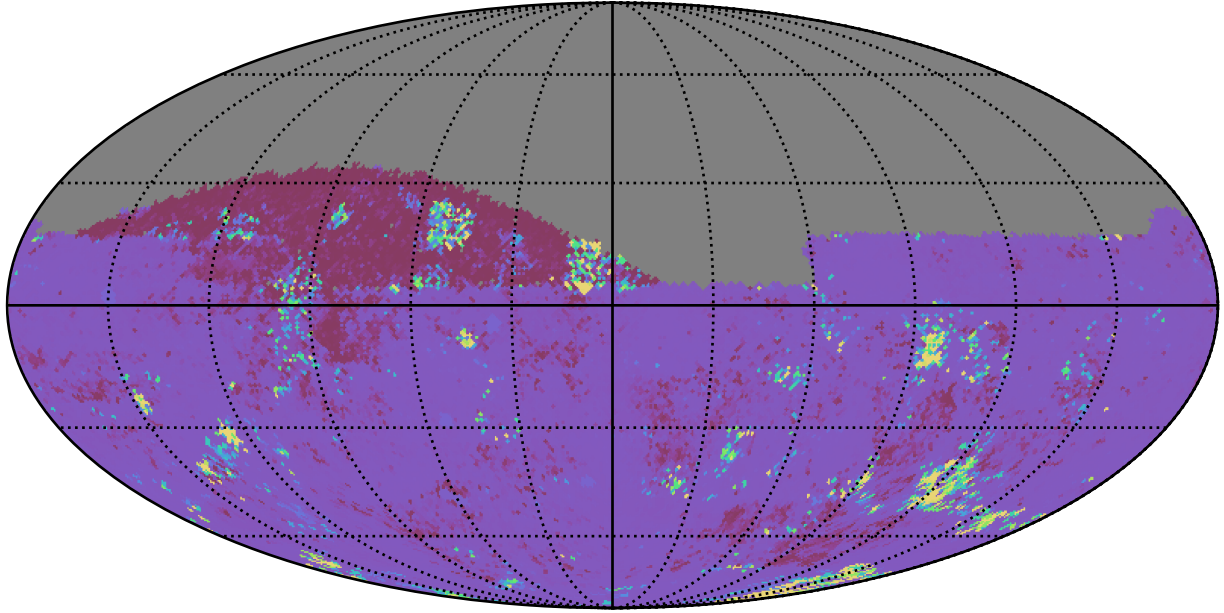
too_elab_heavy_r64_d2_griz_v3.4_10yrs All sky ug bands: 75th Percentile Intranight Timespan
