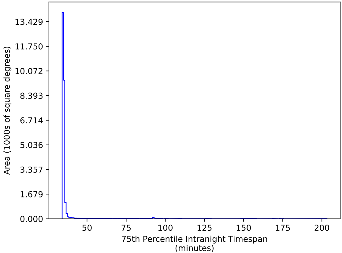
too_elab_heavy_r64_d2_griz_v3.4_10yrs All sky ri bands: 75th Percentile Intranight Timespan
