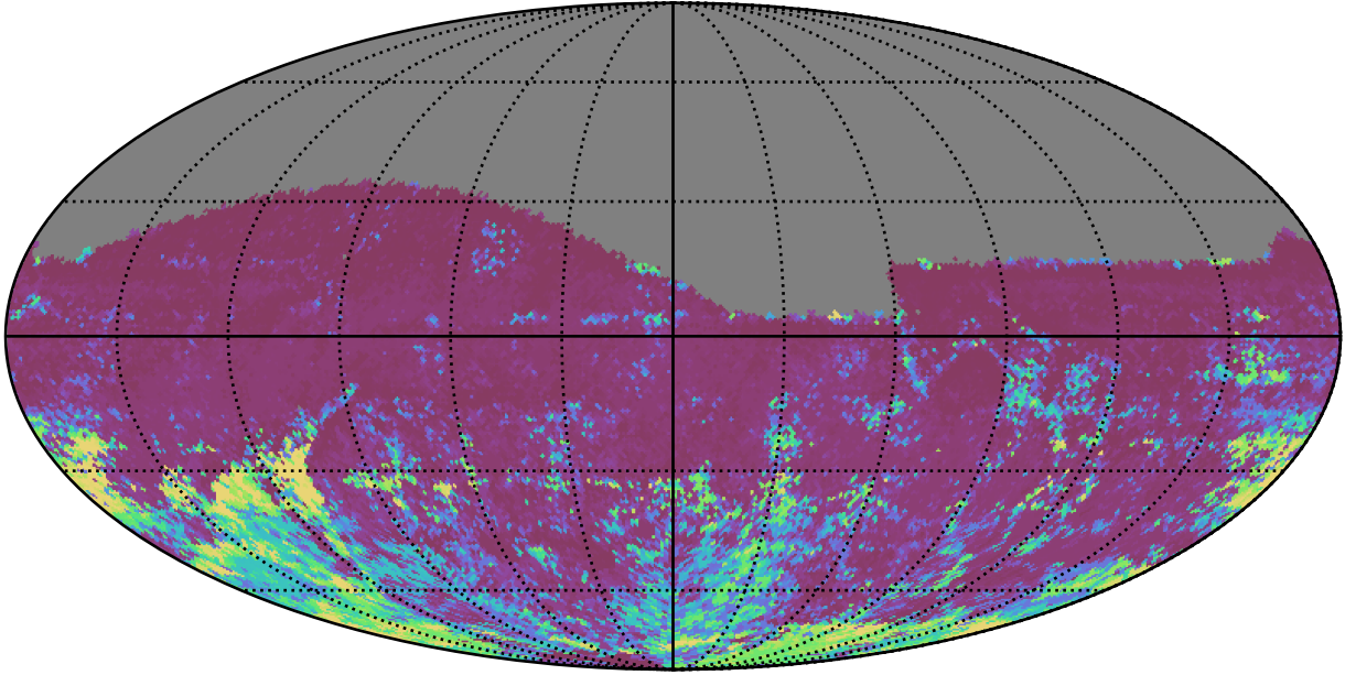
too_elab_heavy_r64_d2_griz_v3.4_10yrs All sky r band: 75th Percentile Intranight Timespan
