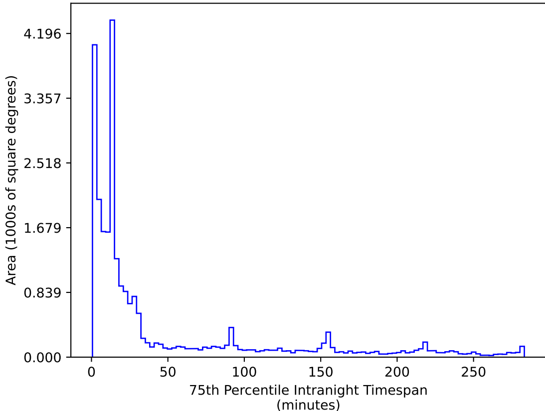
too_elab_heavy_r64_d2_griz_v3.4_10yrs All sky r band: 75th Percentile Intranight Timespan
