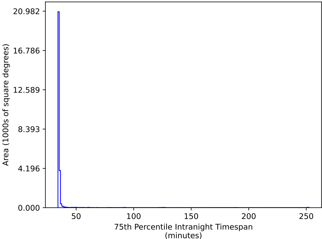
too_elab_heavy_r64_d2_griz_v3.4_10yrs All sky gr bands: 75th Percentile Intranight Timespan
