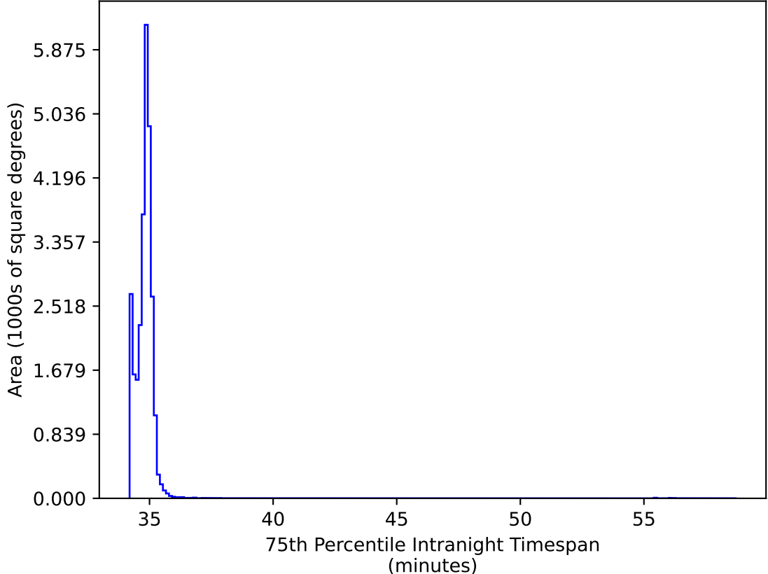
too_elab_heavy_r64_d2_griz_v3.4_10yrs All sky: 75th Percentile Intranight Timespan
