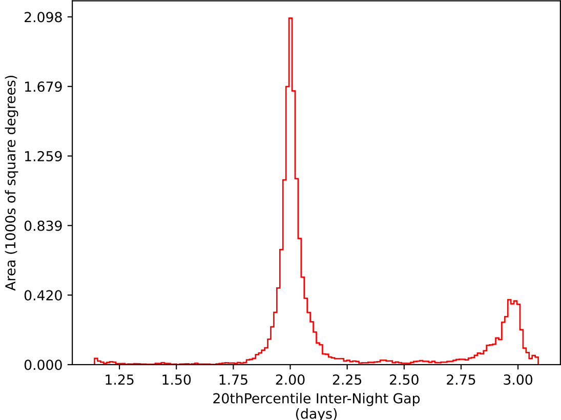
too_elab_heavy_r64_d2_griz_v3.4_10yrs WFD i band: 20thPercentile Inter-Night Gap
