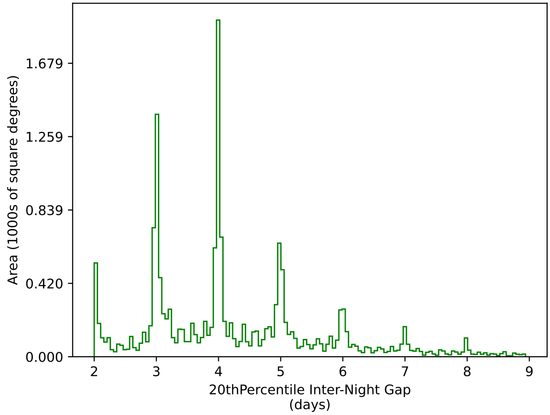
too_elab_heavy_r64_d2_griz_v3.4_10yrs WFD g band: 20thPercentile Inter-Night Gap
