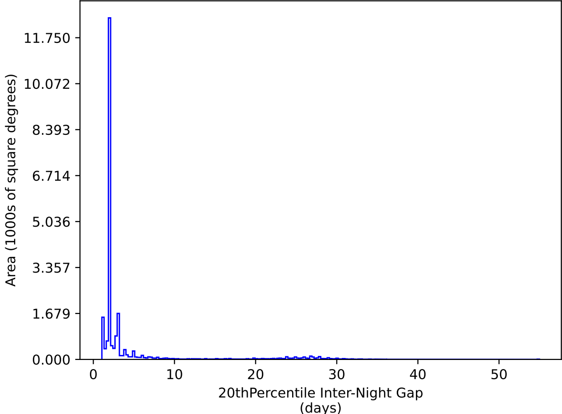
too_elab_heavy_r64_d2_griz_v3.4_10yrs All sky y band: 20thPercentile Inter-Night Gap
