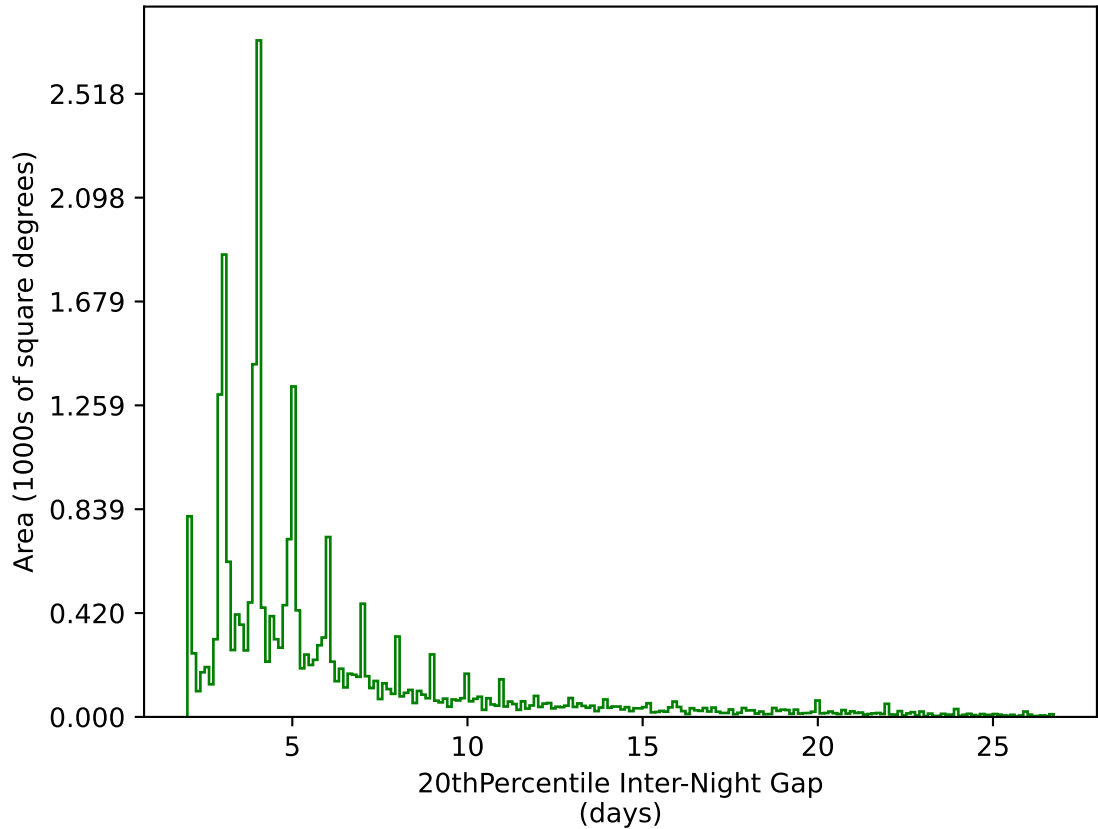
too_elab_heavy_r64_d2_griz_v3.4_10yrs All sky g band: 20thPercentile Inter-Night Gap
