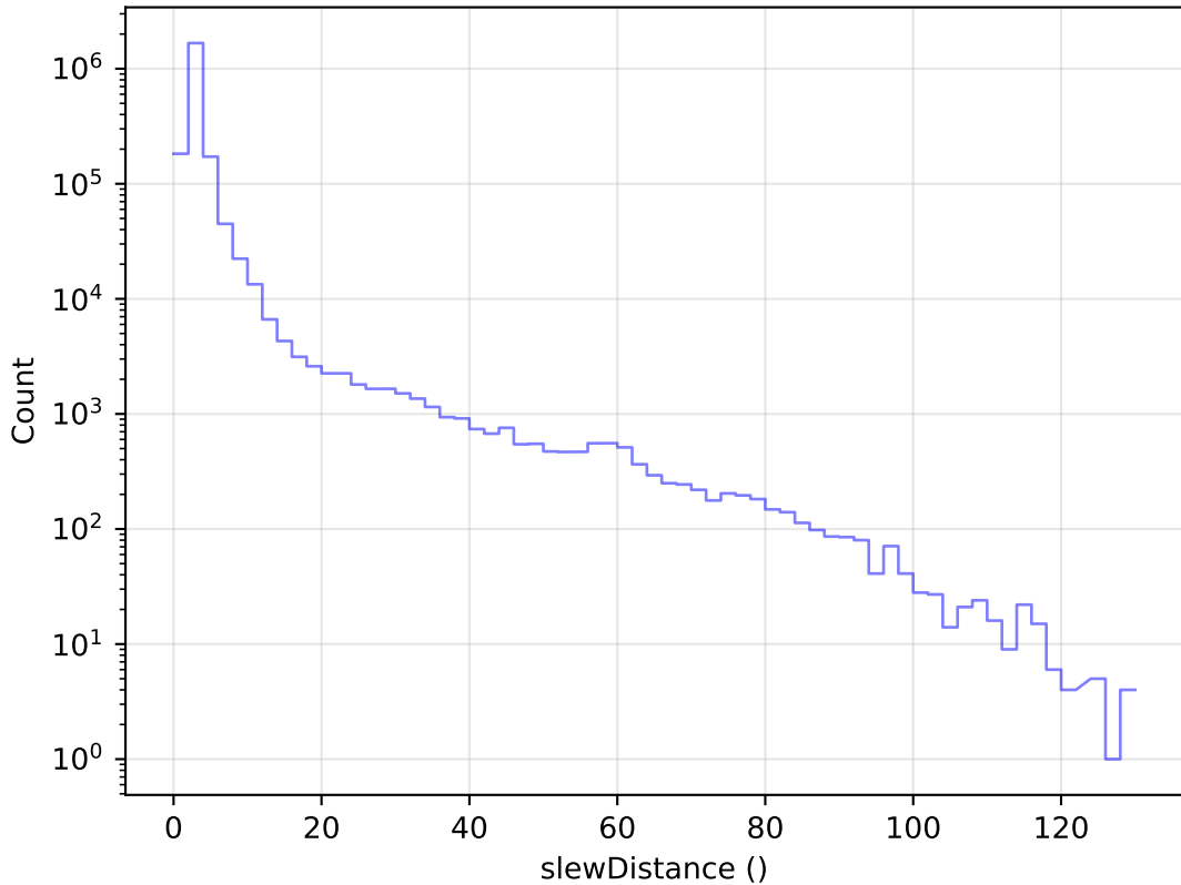
too_elab_heavy_r64_d2_griz_v3.4_10yrs All visits: Slew Distance Histogram
