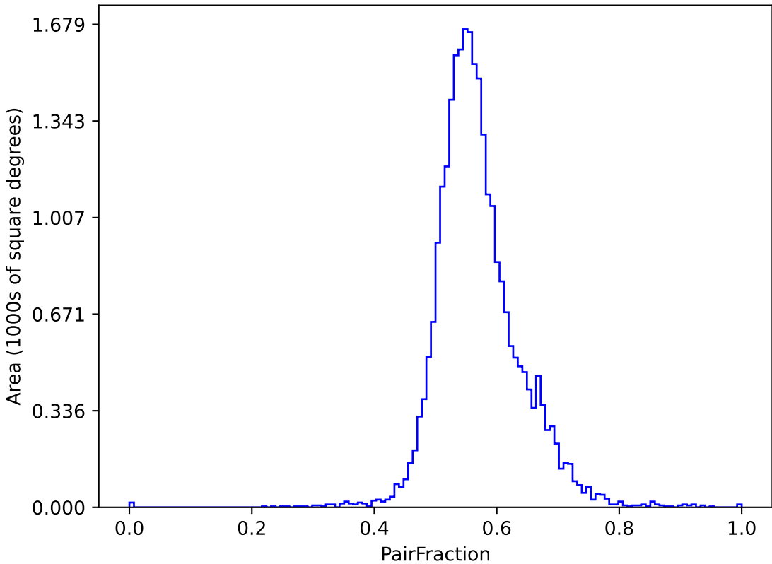
too_elab_heavy_r64_d2_griz_v3.4_10yrs (g or r or i): PairFraction
